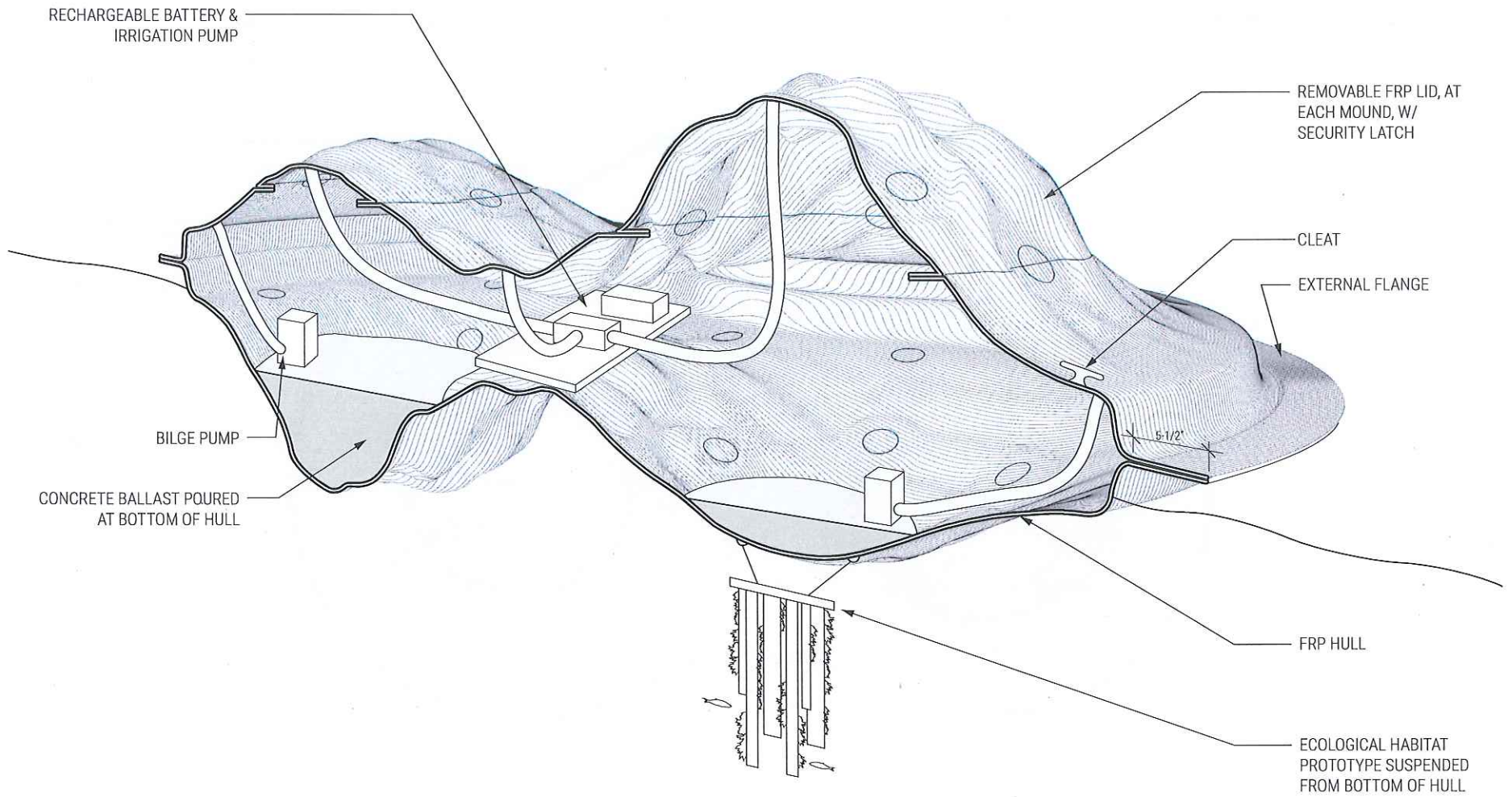
Section Cutaway
